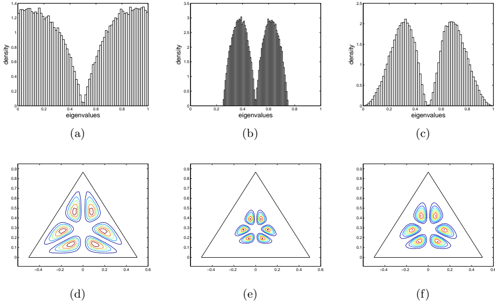
FIGURE 1. Asymptotic measure eigenvalue distribution. First row, from left to right: ( d = 2, b = [1, 0] ), ( d = 2, b = [3/4, 1/4] ), ( d = 2, b = [1, 0, 0, 0] ). Second row: ( d = 3, b = [1, 0, 0] ), ( d = 3, b = [3/4, 1/8, 1/8] ) and ( d = 3, b = [1, 0, 0, 0, 0] ).
