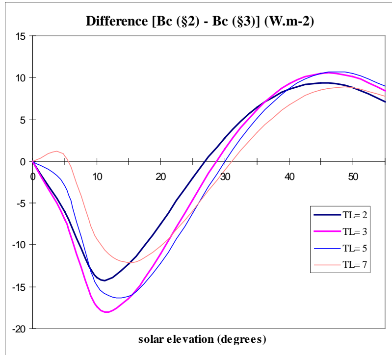
Fig. 9 Difference between Bc_{\text{\$2}} (beam irradiance for clear sky, section 2) and Bc_{\text{\$3}} (beam irradiance for clear sky, section 3), as a function of the solar elevation and T_L(\text{AM2}) , at mean solar distance.
