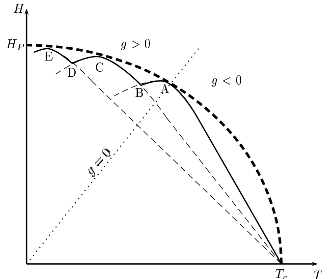
FIG. 2: Schematic field-temperature ( H, T ) phase diagram showing the cascade of Landau levels. The thick dashed curve represents the critical field in the absence of orbital effect. In presence of orbital effect, the critical field is reduced and described by the thin dashed curves which corresponds respectively to the n = 0 , n = 1 and n = 2 Landau levels. The solid line represents schematically the expected transition line between the normal and the superconducting states. The fluctuations are diamagnetic between zero field ( H = 0, T_c ) and B , paramagnetic near the arc AB , then again diamagnetic near the arc BC , etc... The Landau levels are degenerate at points B, D , etc... This schematic picture is relevant for both 2D FFLO superconductors and for 3D ones where the Landau level modulation is realized (scenario b) evoked in the introduction).
