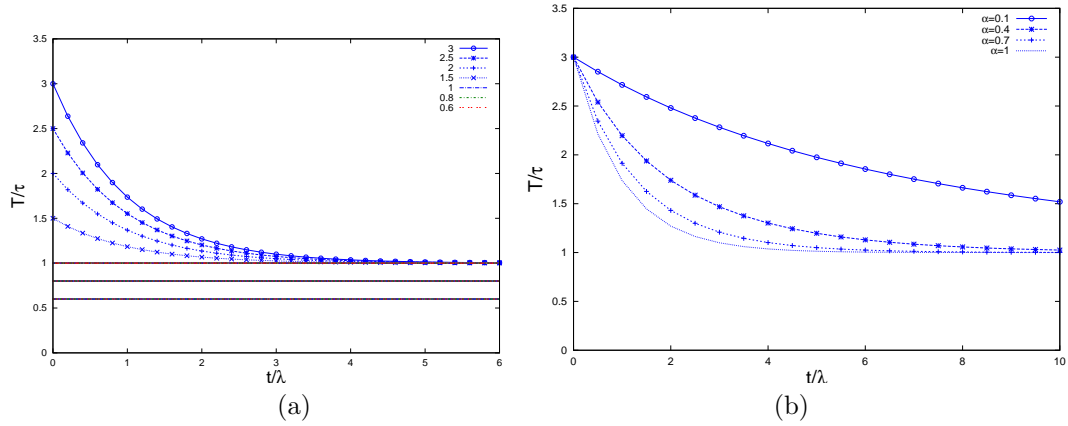
Figure 4: Stress relaxation response (Time is normalized with respect to \lambda .) (a) T/\hat{\tau} for different values of \mu\gamma_0/\hat{\tau} and \alpha = 1 . For \gamma_0 \leq \hat{\tau}/\mu the response is elastic. (b) Evolution of T/\hat{\tau} for \mu\gamma_0/\hat{\tau} = 3 and for increasing values of \alpha (from upper to lower curves).
