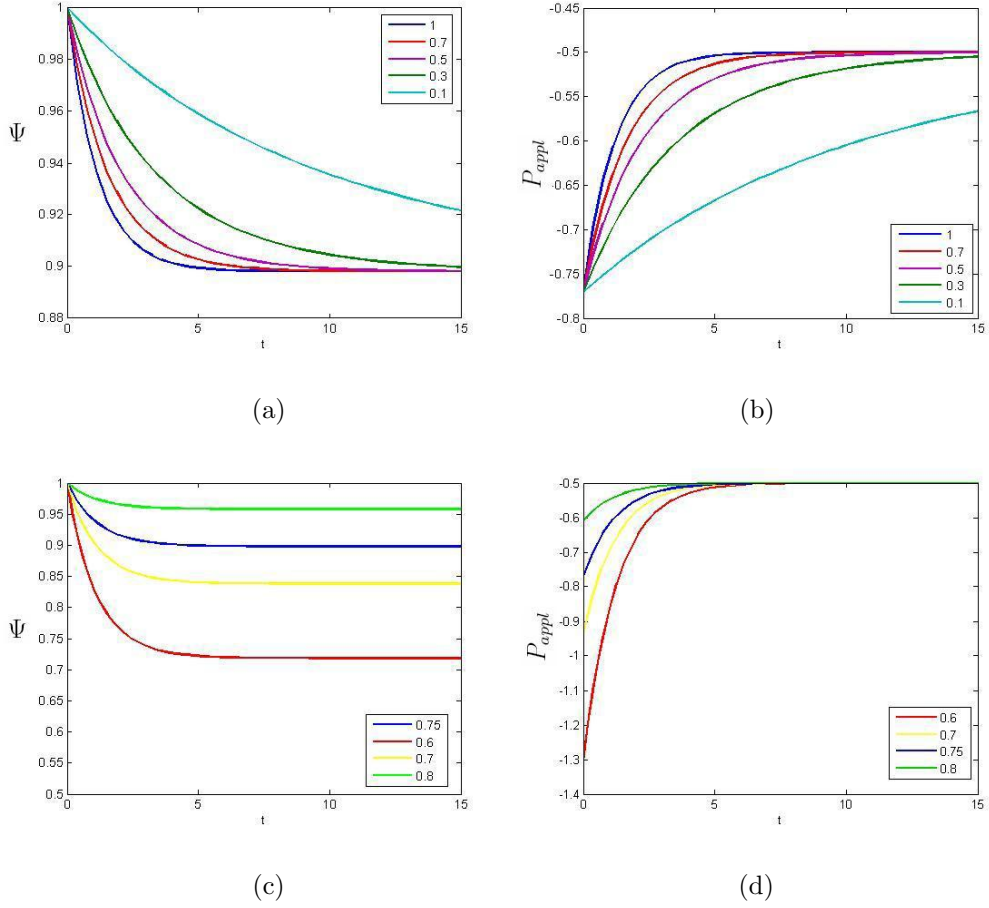
Figure 6: Uniaxial compression for \hat{\tau}/\mu = 0.25 . Time is normalized with respect to \tilde{\eta}/\mu and the applied stress is reported normalized with respect to \mu . In (a,b) \psi_0 = 0.75 and \alpha = 0.1, 0.3, 0.5, 0.7, 1 . In all cases the asymptotic value of \Psi is \Psi_\infty = 0.8981 and P_{appl}/\mu tends to 2\hat{\tau}/\mu = -0.5 . In (c,d) \alpha is fixed to 1 while \psi_0 changes. If \psi_0 > 0.8351 the compression is not strong enough to trigger cell re-organization and therefore \Psi(t) = 1 does not evolve and P_{appl}/\mu is constantly equal to \psi_0^2 - 1/\psi_0 > -0.5 .
