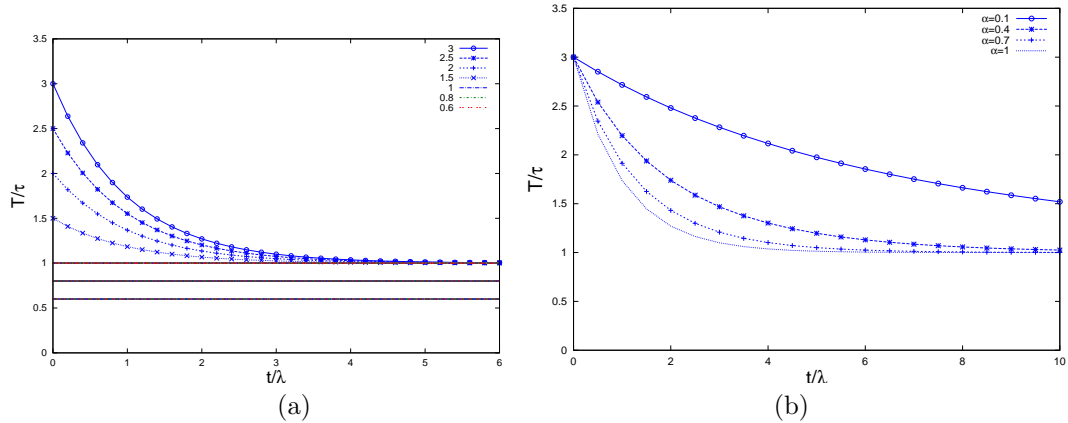
Figure 4: Stress relaxation response (Time is normalized with respect to \lambda .) (a) T/\hat{\tau} for different values of \mu\gamma_0/\hat{\tau} and \alpha = 1 . For \gamma_0 \leq \hat{\tau}/\mu the response is elastic. (b) Evolution of T/\hat{\tau} for \mu\gamma_0/\hat{\tau} = 3 and for increasing values of \alpha (from upper to lower curves).
