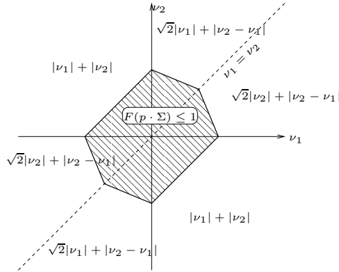
FIGURE 1. Values of F given by (5.1)
