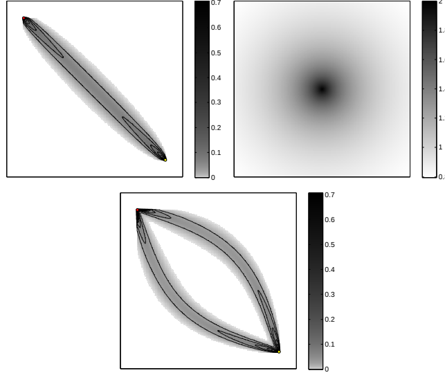
FIGURE 1. Examples of the subgradient computation using our algorithm presented in [4]. On the left, an element of the subdifferential of the geodesic with respect to the metric. The metric is constant, and the geodesic is a straight line. In the middle, we chose a non constant metric \xi(x) = 1/(1.5 - \exp(-d(\mathcal{O}, x))) , where \mathcal{O} is the center of the image. On the right, an element of the subdifferential of the geodesic with respect to the metric given on the second figure.
