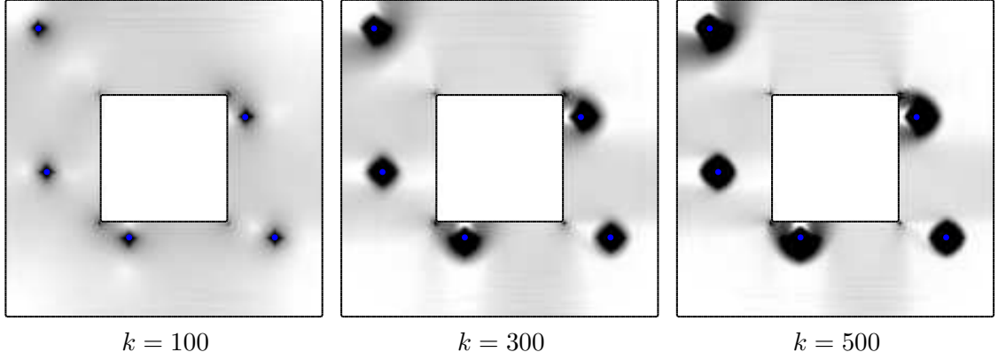
Figure 9: Iterations \xi^{(k)} computed for a domain \Omega with a hole and with P = 5 landmarks.
