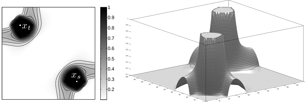
Figure 5: 2D and 3D display of the optimal metric \xi^* .
