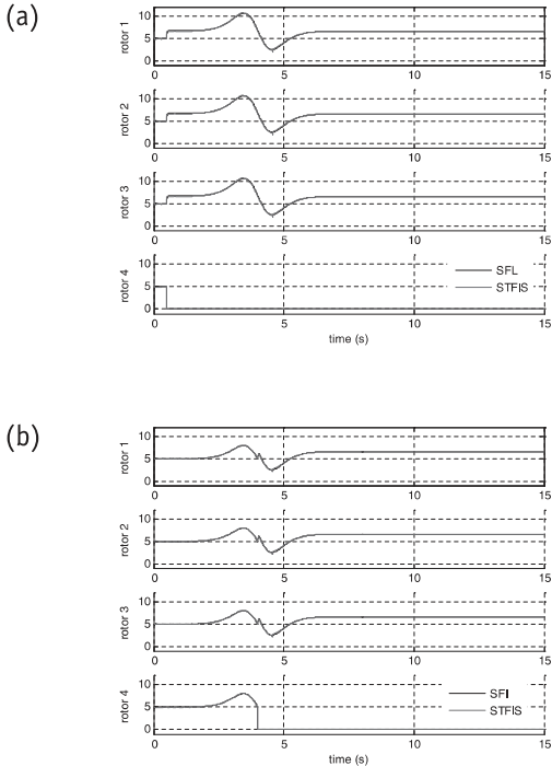
Fig. 6. XSF Forces in the case of motor 4 failure at t = 0.5 \text{ s} (a) and t = 4 \text{ s} (b).
