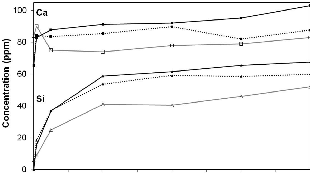
Figure 7. Ca (squares), Si (triangles), P (circles) and Zn (cross) concentrations in DMEM after interaction with bioactive glasses. Undoped sample is in grey line, Zn1 in dotted lines and Zn5 in straight lines.
