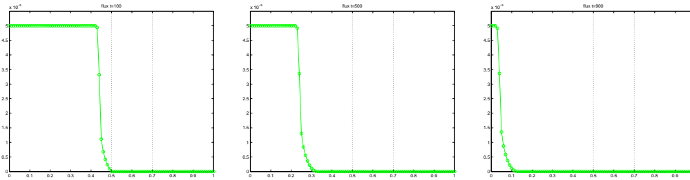
Figure 6: Oil-flux profiles for t = 100, t = 500, t = 900
