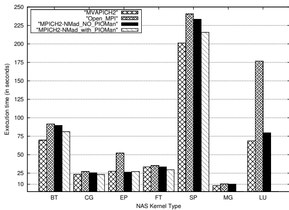
(c) 32/36 Processes
