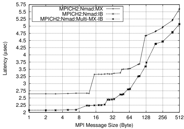
(a) Latency
