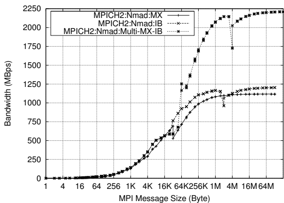
(b) Bandwidth
