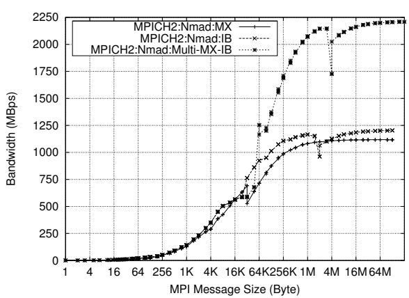
(b) Bandwidth
