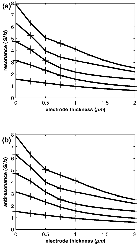
FIG. 4. (a) Resonance frequencies vs electrode thickness. (b) Antiresonance frequencies vs electrode thickness (solid line: analytical results; +: anticipation polynomial method). M=15 .
