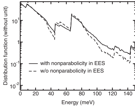
FIG. 9. Distribution function as a function of the energy for two EES models. Solid line: with NP in EES; Dashed line: without NP in EES. The energy reference of both curves is the bottom of the first subband.
