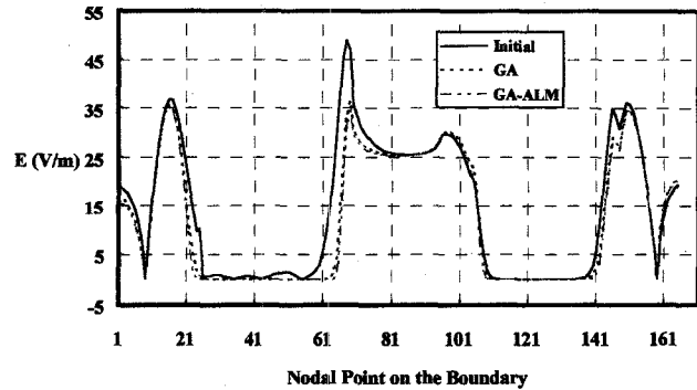
Fig. 2. E-field (initial geometry, geometry obtained with GA and passed to ALM and the final result obtained with GA-ALM).
