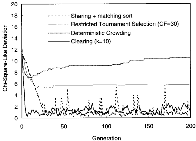
Fig. 13. Chi-square-like deviation of the niching GA's investigated on function F4 . The population size is N = 100 .
