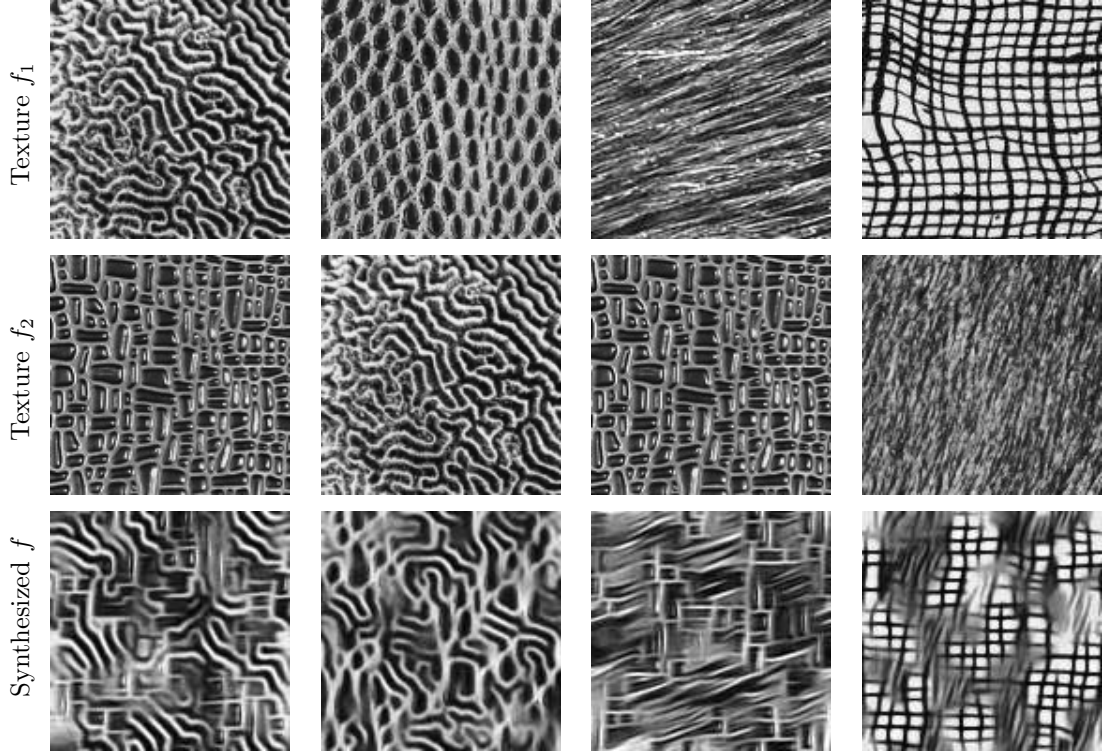
Figure 12: Examples of texture mixing with sparsity s = 4 .
