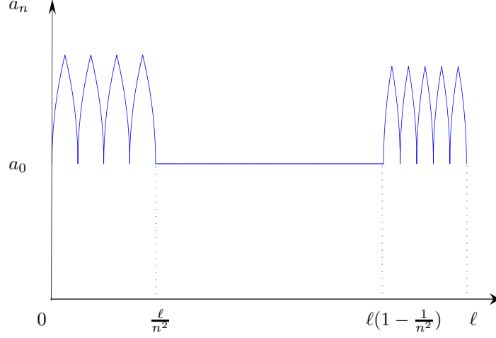
FIGURE 2. Representation of a minimizing sequence
