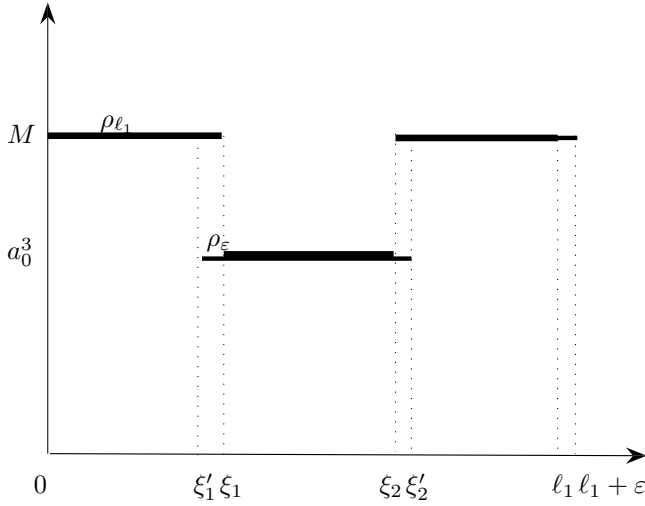
FIGURE 4. Representation of functions \rho_{\ell_1} and \rho_\varepsilon
