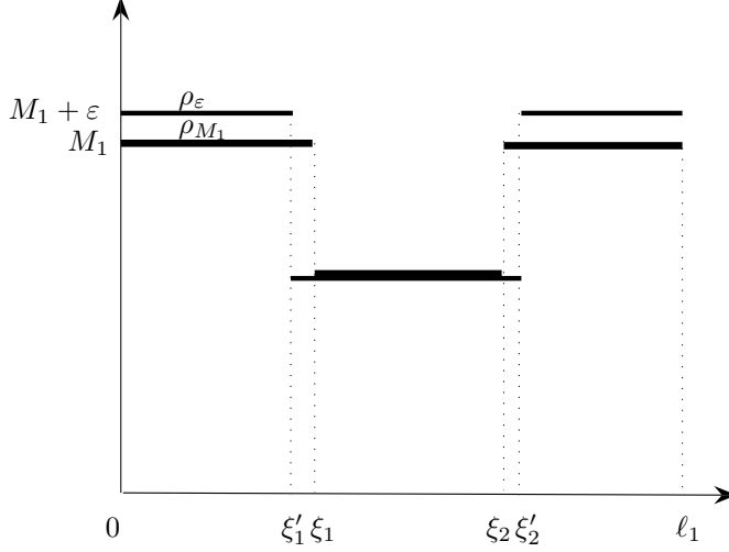
FIGURE 3. Representation of functions \rho_{M_1} and \rho_\varepsilon
