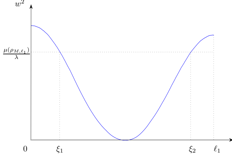
FIGURE 1. Representation of the eigenfunction w^2 and construction of \xi_1 and \xi_2
