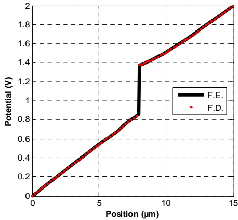
Fig. 1 Potential along one symmetry axis of the cell at 5 MHz computed with both methods.
