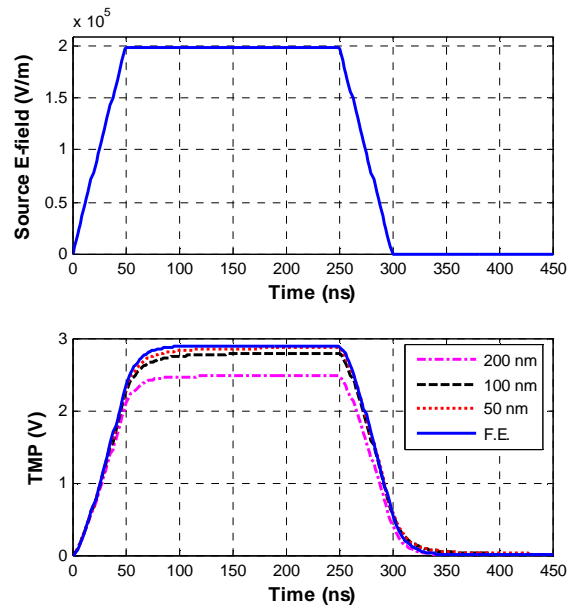
Fig. 2 Time-transient response of the cell (Max. source E-field: 2.10^5 V/m).
