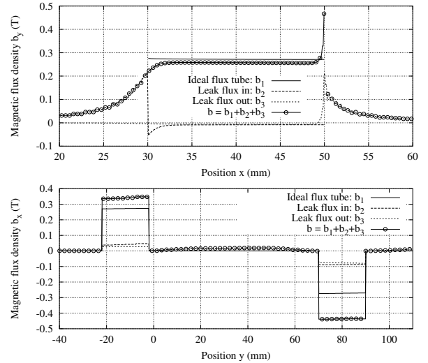
Fig. 9. Magnetic flux density along the top surface of the I-core (entering the air gap; top) and through the horizontal legs of the electromagnet (bottom) for the ideal flux tube ( \mathbf{b}_1 ) and the inner ( \mathbf{b}_2 ) and outer ( \mathbf{b}_3 ) leakage fluxes; their addition gives the complete solution ( \mathbf{b} ).
