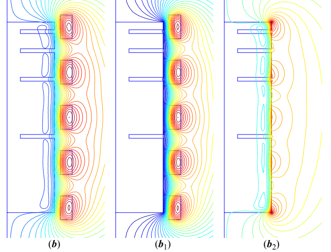
Fig. 11. Magnetic flux lines for the conventional FE solution \mathbf{b} , the reference solution \mathbf{b}_1 and the perturbation solution \mathbf{b}_2 ; system with a conductive non-magnetic core (aluminium) [8].
