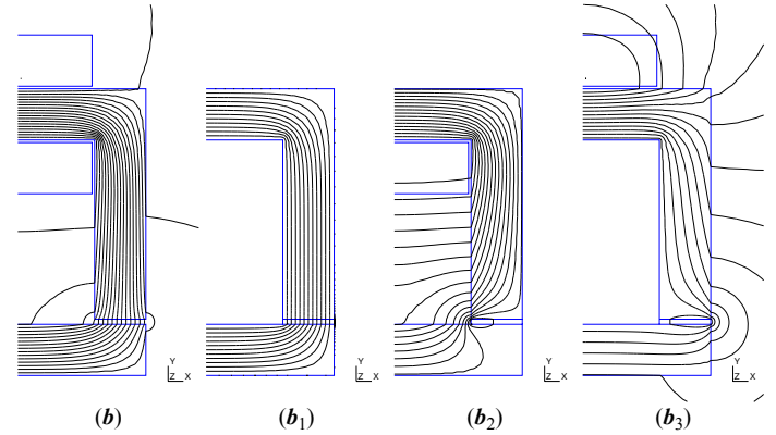
Fig. 8. Field lines of the complete solution ( \mathbf{b} ), in the ideal flux tube ( \mathbf{b}_1 ) and in the perturbation problems with the inner ( \mathbf{b}_2 ) and outer ( \mathbf{b}_3 ) leakage fluxes (from left to right; the perturbation flux between two consecutive field lines is 4 times lower than for the source flux).
