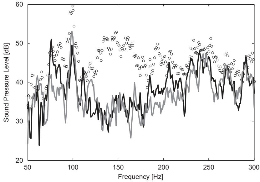
Fig. 9. Sound pressure level measured at the observation microphones with and without the DAB: \circ SPL control off; \text{—} SPL with DAB on secondary monopole-like sources placed at 20 cm from the partition wall; and \text{—} SPL with DAB on secondary dipole-like sources placed at 35 cm from the partition wall.
