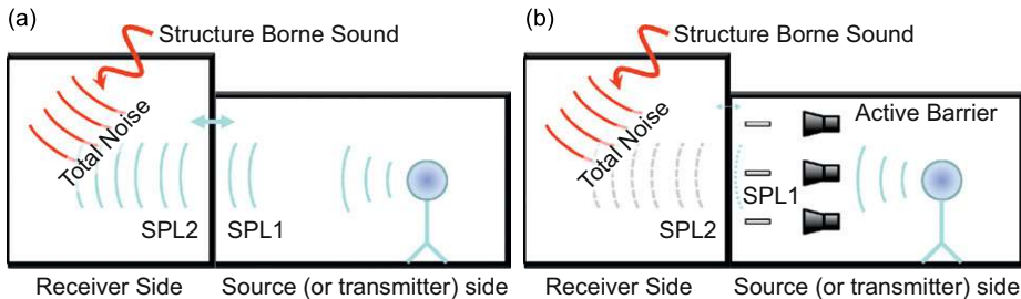
Fig. 1. Diagram of the approach presented in this paper. Comparison between the standard condition (a) and condition (b) with the active noise control system designed to minimize the sound pressure on the right (source) side of the partition.
