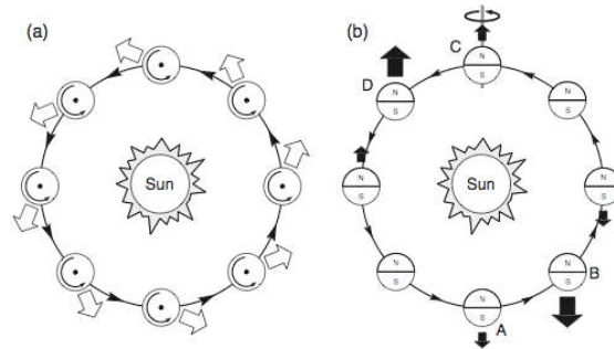
Fig. 22. The diurnal (left) and seasonal (right) Yarkovsky effects. Depending on the prograde (resp. retrograde) spin axis direction the force will secularly decrease (resp. increase) the semi-major axis of the asteroid (diurnal). In case of zero obliquity (purely seasonal) one always has da/dt \leq 0 . (Copyright GSFC NASA).
