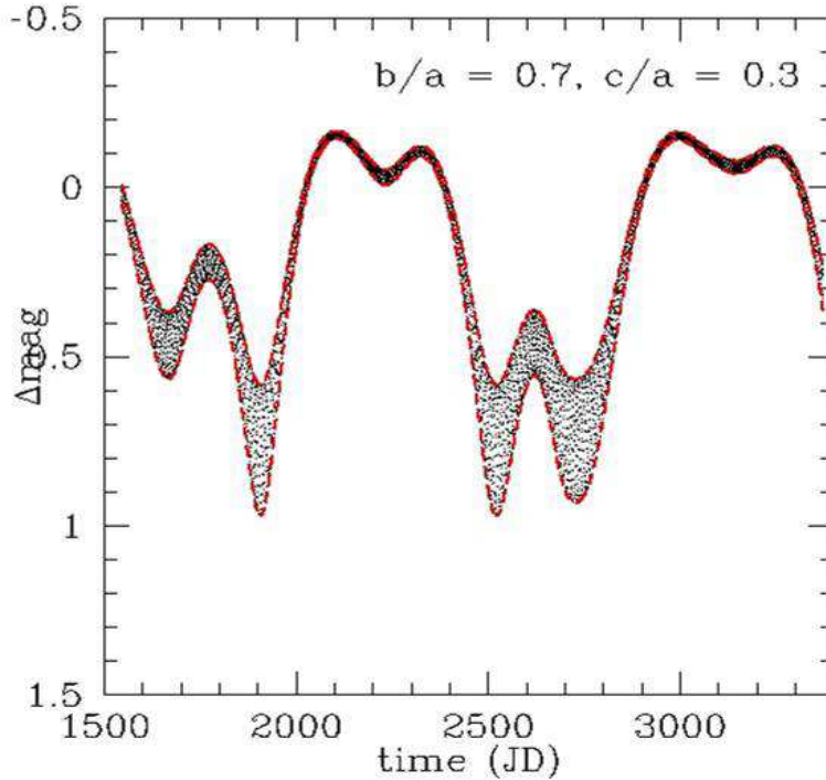
Fig. 13. The same as Fig. 10, but this time for an object having the same pole ( \lambda = 30^\circ , \beta = 60^\circ ), but a more elongated shape: b/a = 0.7 , c/a = 0.3 .
