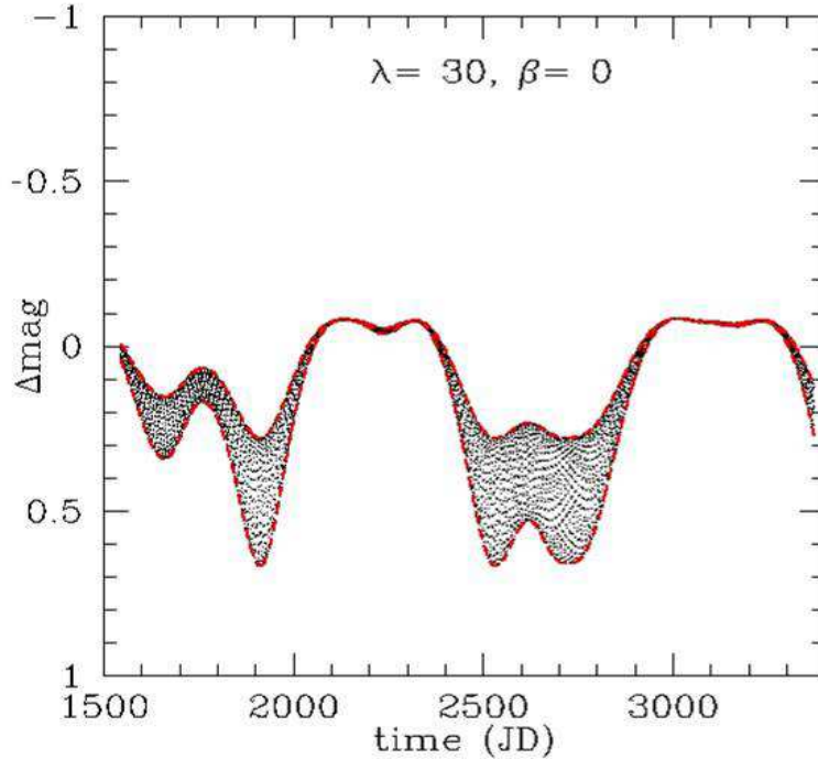
Fig. 12. The same as Fig. 10, but this time the ecliptic latitude of the asteroid’s pole is \beta = 0^\circ .
