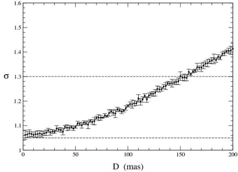
Fig. 5. Standard deviation \sigma (in pixels) of signals produced by an ideal spherical and homogeneously emitting object seen at zero phase angle, as a function of its apparent diameter D . The bar corresponds to the standard deviation of \sigma . due to photon statistics.
