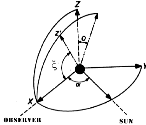
Fig. 9. Graphical explanations of the aspect ( \xi ) and the obliquity ( o ) angles. The angle \alpha in this figure is the phase angle. Vector \mathbf{Z}' is the direction of the positive spin.
