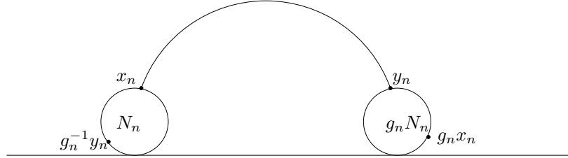
FIGURE 4. The horoball approximation N_n and its translate by g_n
