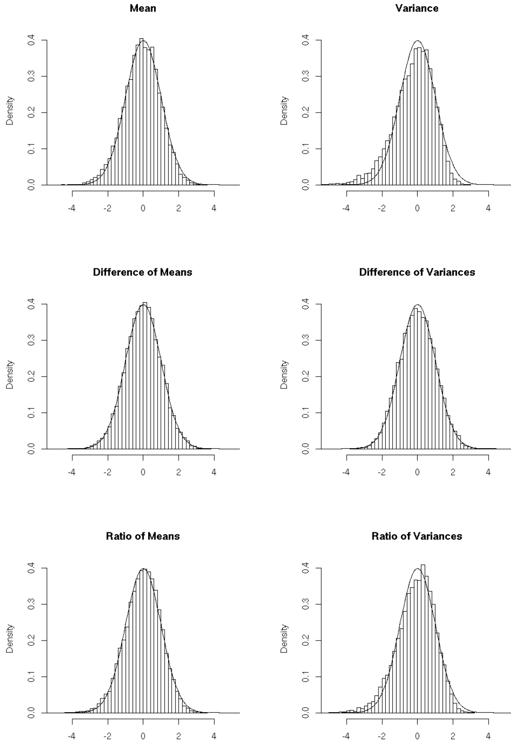
9 Figure 3: Histograms of m = 10000 replications of \frac{\hat{\theta}(\mathbf{Y}) - \theta}{\hat{\sigma}_{\hat{\theta}}(\mathbf{Y})} for \theta = \mu, \sigma^2, d_{\mu}, d_{\sigma^2}, r_{\mu} and r_{\sigma^2} . The simulation has been done as follows: n = n^{(1)} = n^{(2)} = 500, Y^{(1)} \rightsquigarrow \mathcal{E}(1), Y^{(2)} \rightsquigarrow \mathcal{E}(1) .
