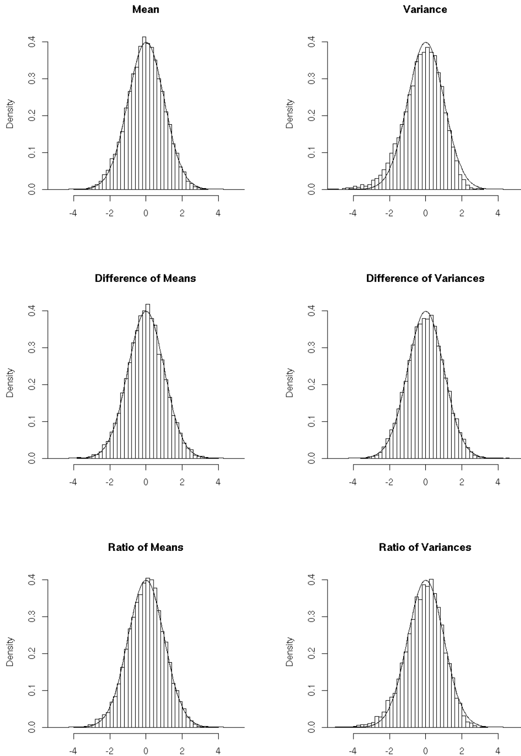
8 Figure 2: Histograms of m = 10000 replications of \frac{\hat{\theta}(\mathbf{Y}) - \theta}{\hat{\sigma}_{\hat{\theta}}(\mathbf{Y})} for \theta = \mu, \sigma^2, d_{\mu}, d_{\sigma^2}, r_{\mu} and r_{\sigma^2} . The simulation has been done as follows: n = n^{(1)} = n^{(2)} = 500, Y^{(1)} \rightsquigarrow \chi^2(5), Y^{(2)} \rightsquigarrow \chi^2(5) .
