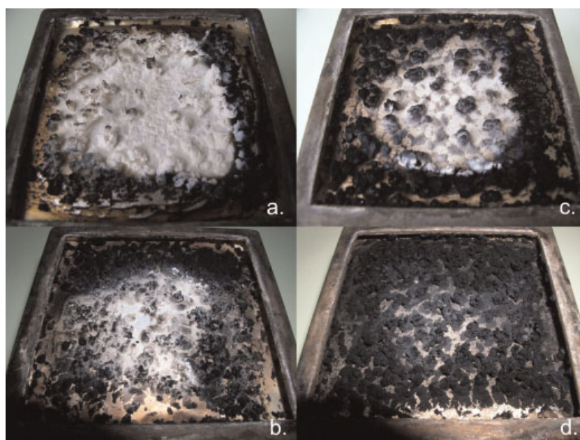
Figure 11. Photographs of char residues after cone calorimeter experiments from samples with PMMA 95% and (a) AluC 5%, (b) Alu-PDMS 5%, (c) Alu-PET 5%, (d) Alu-TER 5%. This figure is available in color online at www.interscience.wiley.com/journal/pat
