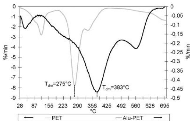
Figure 3. DTG curves of Alu-PET and PET at a heating rate of 10^\circ\text{C min}^{-1} .
