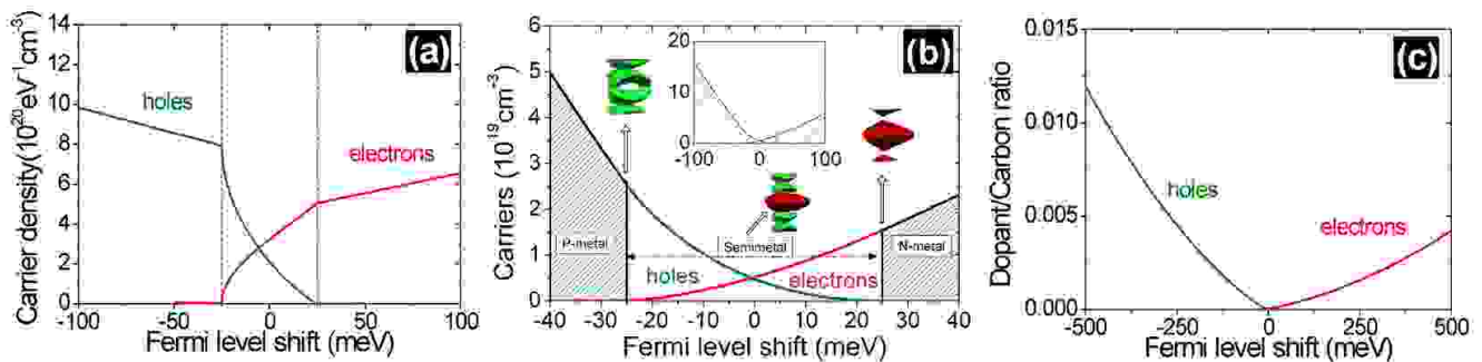
FIG. 10: Doping dependence of (a) the electron and hole carrier density (b) the number of electrons and holes and (c) the stoichiometric dopant to carbon ratio. The red(green) lines represent electron(hole) carriers.
