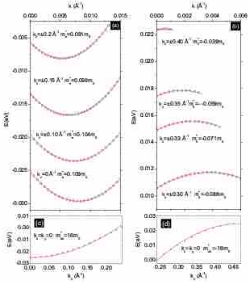
FIG. 8: Evaluation of the in-plane (a) electron and (b) hole masses around K and H , respectively. The dispersions along the parabolas depicted by points 1 – 2 – 3 in Fig. 7 are taken for evaluation of the masses. The effective masses perpendicular to the layers in z direction are shown in (c) for electrons and in (d) for holes. \square correspond to TB-GW values and the red lines are parabolic fits.
