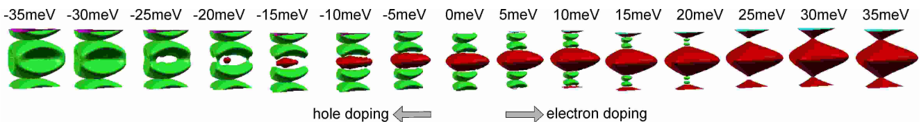
FIG. 11: The Fermi surface of doped graphite in the dilute limit for electron doping and hole doping. The red(green) surfaces are the electron(hole) pockets of the Fermi surface. It is clear that at \pm 25 meV we have a semi metal to metal transition.
