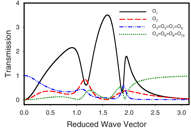
FIG. 2. (Color online) Output-signal intensities as a function of kd . The results were obtained for k_0d = \pi/2 .
