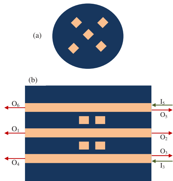
FIG. 1. (Color online) Sketch of the considered fiber structure. (a) The entrance of the four external input channels within the center at the rear of the main output channel. (b) The transversal cut of the fiber showing the central output hole and two of the four external input and output holes, as well as the cavities responsible for the resonant coupling between the input and output channels. The input intensities are labeled as I_i with i=3, 5, 7, 9 and the output amplitudes as O_i with i=1-10 .
