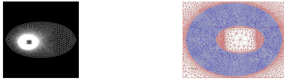
FIGURE 5.1. 2D mesh with 8554 vertexes and 17016 triangles.
