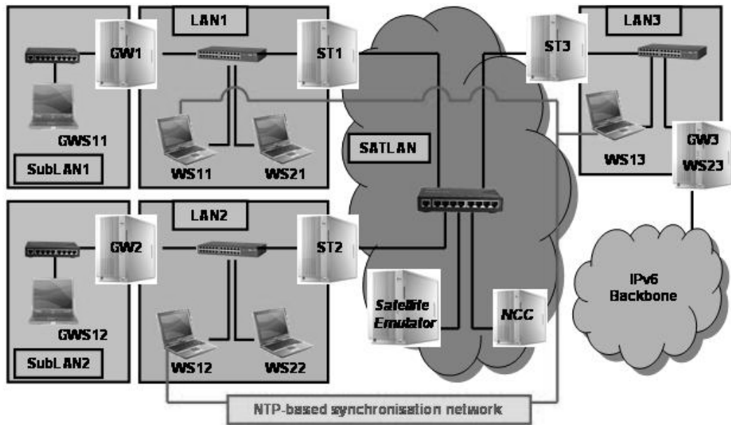
Figure 6: SATIP6 testbed.
