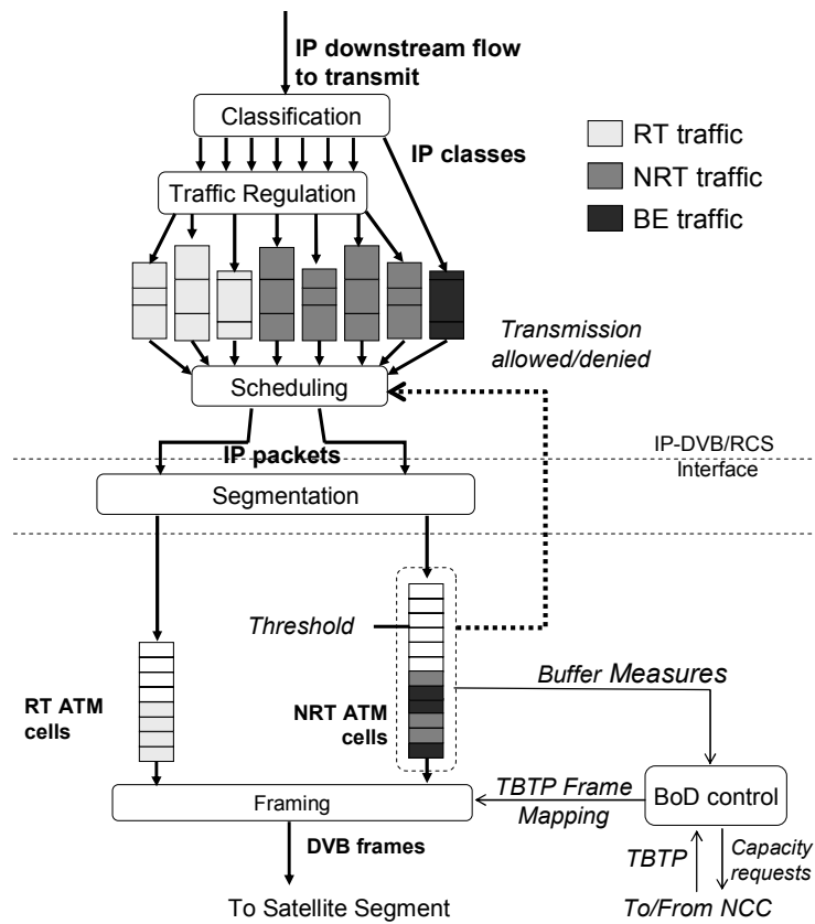
Figure 5: QoS Architecture in the ST.
