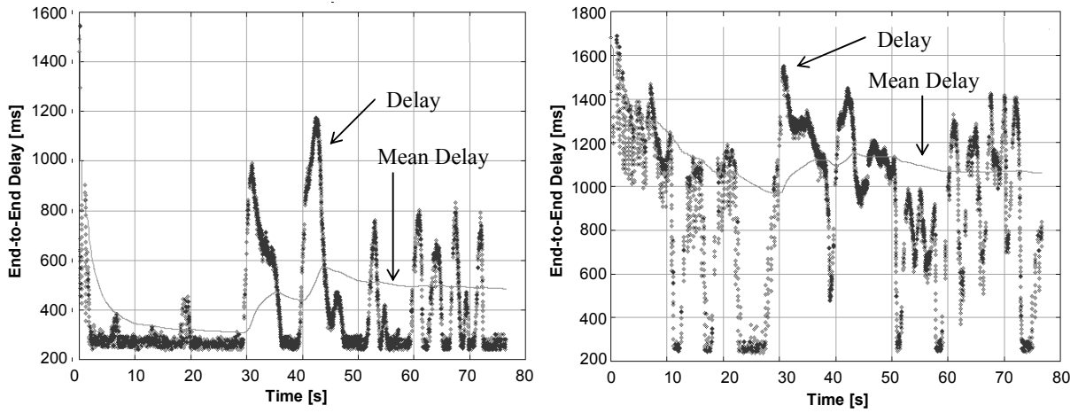
Figure 8: End-to-end delay (dotted) and mean delay (plain) graphs for Xvid video profile; (a) FCA = 300 kbps, (b) FCA = 0 kbps.
