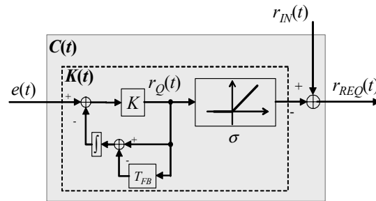
Figure 4: ST BoD Controller.
