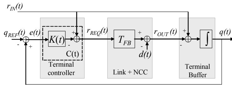
Figure 3: Model of the BoD control system.
