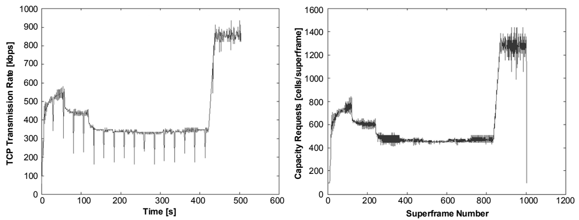
Figure 7: a) Measured TCP throughput during congestion; b) Associated capacity requests.
