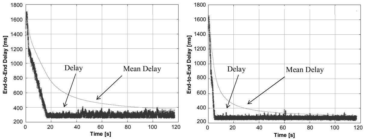
Figure 9: End-to-end delay (dotted) and mean delay (plain) graphs for MPEG video profile; (a) FCA = 0 kbps, (b) FCA = 300 kbps.
