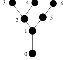
Figure 5: 3,4,6 are leaves; 1, 2 and 5 are nodes, 2 and 5 are uppermost; branches are e.g. Br(2 \rightarrow 1) or Br(6 \rightarrow 1) .
