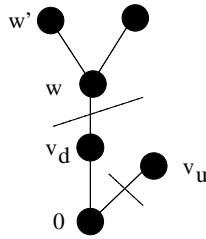
Figure 2: Admissible cut.
