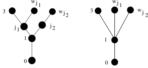
Figure 7: Case (i-a). \mathbb{T} and \check{\mathbb{T}} .
