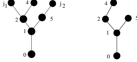
Figure 9: Case (i-c). \mathbb{T} and \tilde{\mathbb{T}} .
