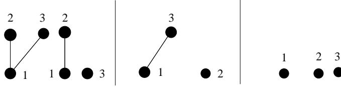
Figure 4: Example 2.12. From left to right: \mathbb{T}_1^\sigma, \mathbb{T}_2^\sigma ; L_{\{1\}}\mathbb{T}_1^\sigma \otimes R_{\{1\}}\mathbb{T}_1^\sigma ; L_{\{1,2\}}\mathbb{T}_1^\sigma \otimes R_{\{1,2\}}\mathbb{T}_1^\sigma
