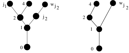
Figure 8: Case (i-b). \mathbb{T} and \check{\mathbb{T}} .
