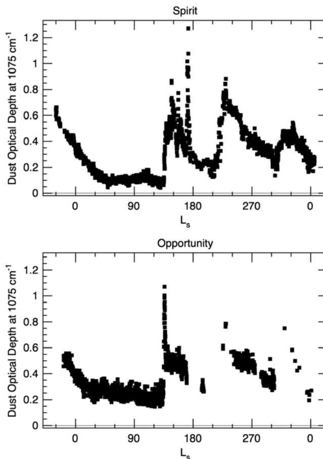
Figure 6. Dust optical depth at 1075 \text{ cm}^{-1} ( 9.3 \mu\text{m} ) as function of season for the Mars Exploration Rovers (top) Spirit and (bottom) Opportunity as retrieved by Smith et al. [2006] using Mini-TES spectrometer observations. The data were obtained during the same year than the SPICAM data discussed in this paper. The fluctuations of atmospheric dust optical depth appear to be correlated with the density variations in the upper atmosphere observed by SPICAM and shown in Figure 4. From Smith et al. [2006].
