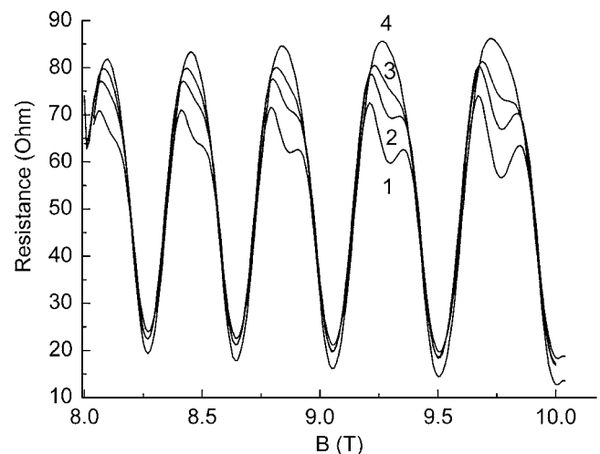
FIG. 6. High magnetic field part of the magnetoresistance R for sample 3 irradiated with a dose of 1 \times 10^6 rad and measured at different temperatures T (K): (1) -0.30 , (2) -1.17 , (3) -2.00 , and (4) -3 .
