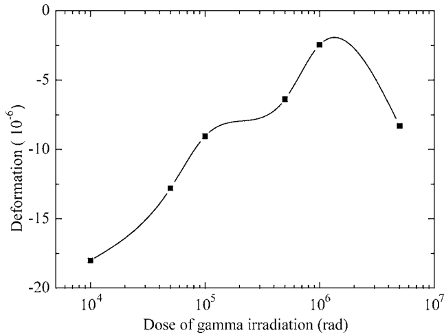
FIG. 1. Irradiation dose dependence of elastic strains in the AlGaIn layer of AlGaIn/GaN heterostructure 1 with the \text{Si}_3\text{N}_4 passivation layer.
