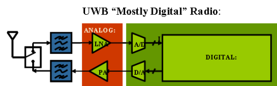
Fig. 7. Illustration of Mostly Digital radio
