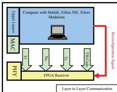
Figure 8. PHY and MAC Layer interface.
