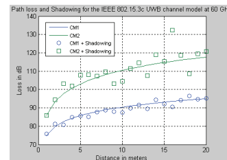
Figure 2. Illustration of the shadowing effect and the path loss for the IEEE 802.15.3c channel model at 60 GHz
