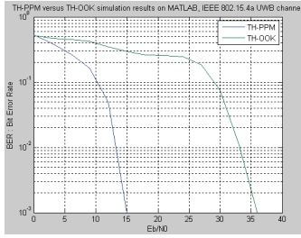
Figure 1. IR-UWB modulation according to BER/ E_b/N_0 in IEEE 802.15.4a UWB channel.
