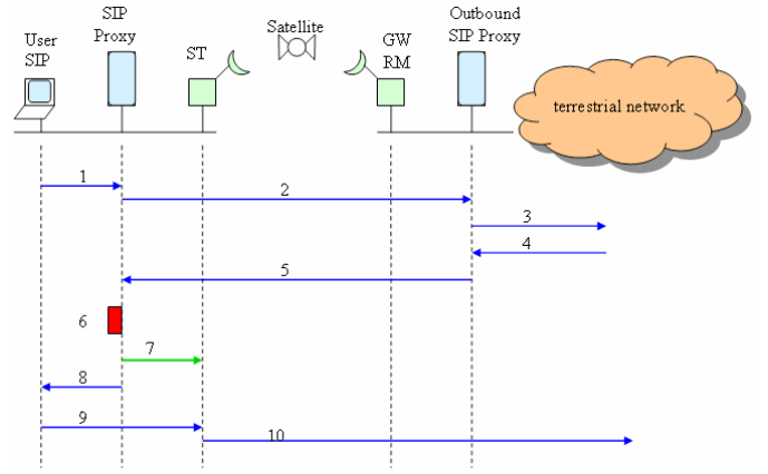
Fig 6. SIP-based anticipation in the ST side
