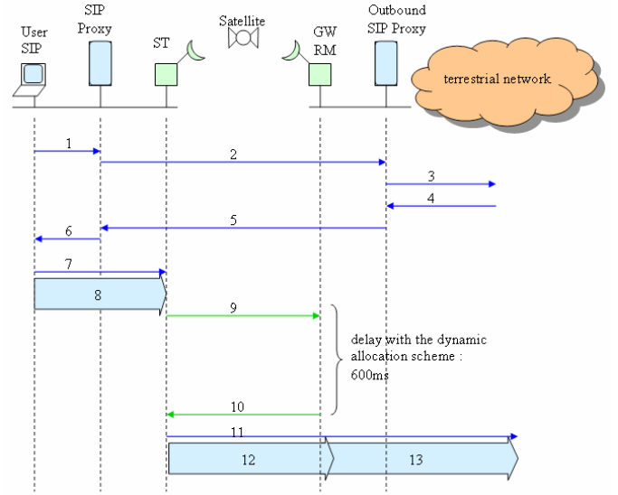
Fig 2. SIP session with a dynamic allocation scheme in satellite system
