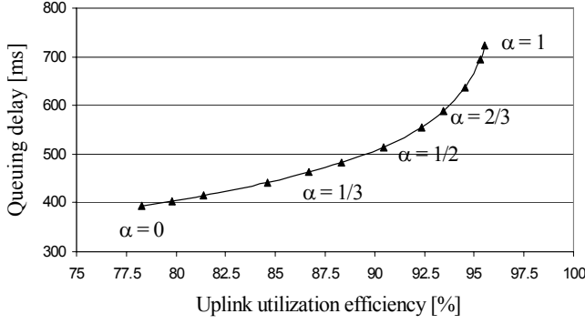
Fig 5. Queuing function of utilization
