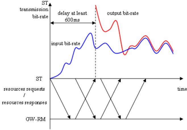
Fig 1. Beginning of a multimedia flow with a dynamic allocation scheme
