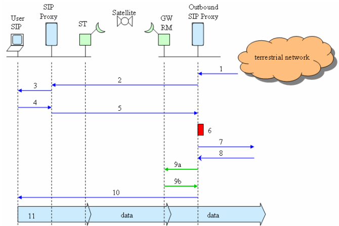
Fig 4. SIP-based provision in satellite system (remote initiation)
