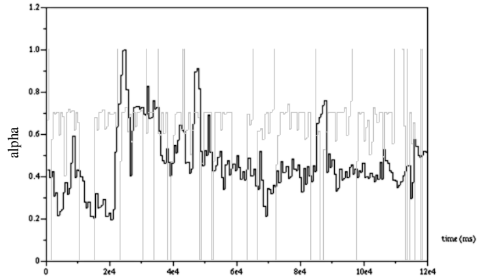
Fig 7. Evolution of \alpha parameter for H.264 codec and GSM codec
