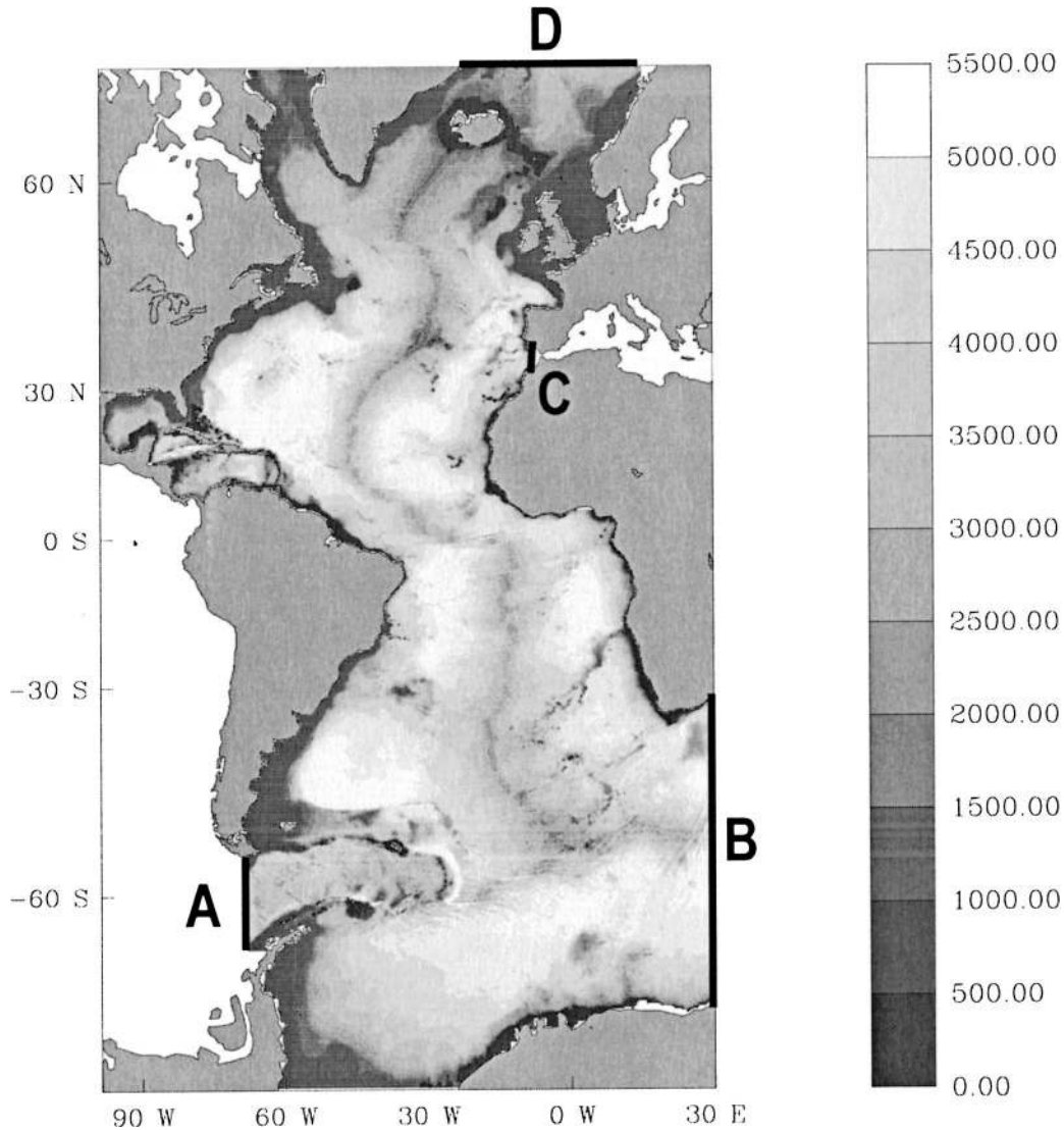
FIG. 1. Model bathymetry (m) and domain. Black lines locate the four open boundaries.
