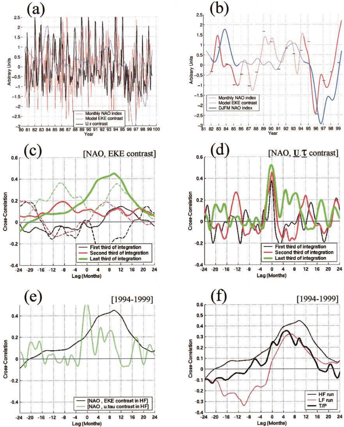
FIG. 5. (a) Normalized anomalies (with respect to the whole time series) of the following quantities in the HF simulation: monthly NAO index (red; Hurrell 1995), meridional contrast of EKE (blue) and of the energy input by the wind, i.e., (\mathbf{u} \cdot \boldsymbol{\tau})_{\text{North}} - (\mathbf{u} \cdot \boldsymbol{\tau})_{\text{South}} , where \mathbf{u} and \boldsymbol{\tau} are the monthly surface model velocity and wind stress, respectively. (b) Blue and red lines from (a) after low-pass filtering. The 1994–99 period from which (c), (d), (e), and (f) were built is highlighted by thick lines. The 1982–85 period is also highlighted. (c) Cross correlations C(t) between the monthly NAO index and the EKE contrast over the three thirds of the period of 1980–99 in the HF simulation. Plain and dashed lines correspond to HF and PF runs, respectively. In every panel, NAO index leads at positive lags. (d) Cross correlation between the NAO index and the meridional contrast of the energy input by the wind during the three thirds of the HF integration. (e) Cross correlation between the NAO index and the EKE contrast (black line) and between the NAO index and the meridional contrast of the energy input by the wind in the HF run over the period of 1994–99 [green corresponds to the latest thick lines in (a) and (b)]. (f) Cross correlation between the NAO index and the EKE contrast diagnosed from the HF run (thin black line), from the LF run (red line), and from T/P data (thick black line) over the period of 1994–99.
