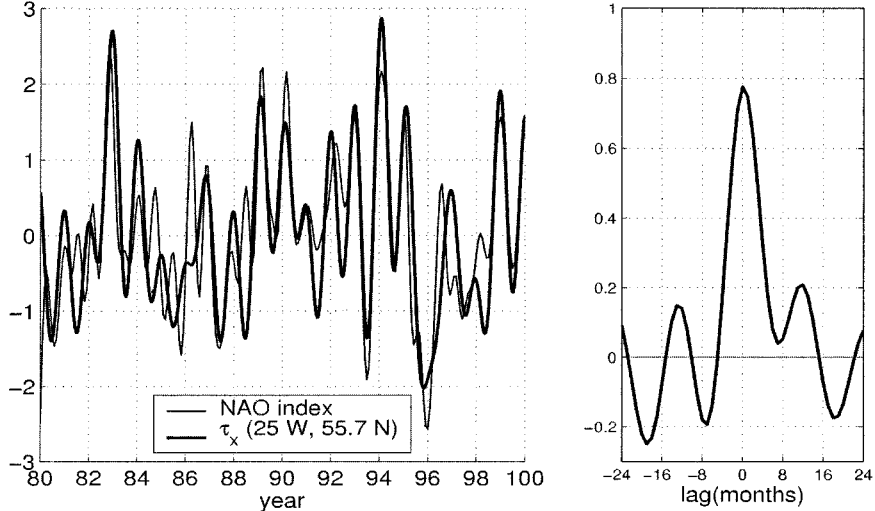
FIG. 6. (left) Evolution of the normalized NAO index thin line and the normalized anomaly of the zonal wind stress at 55.7°N, 25°W throughout the HF integration thick line. The NAO index is taken from Hurrell (1995). (right) Lagged correlation between the NAO index and the wind stress at the same location.
