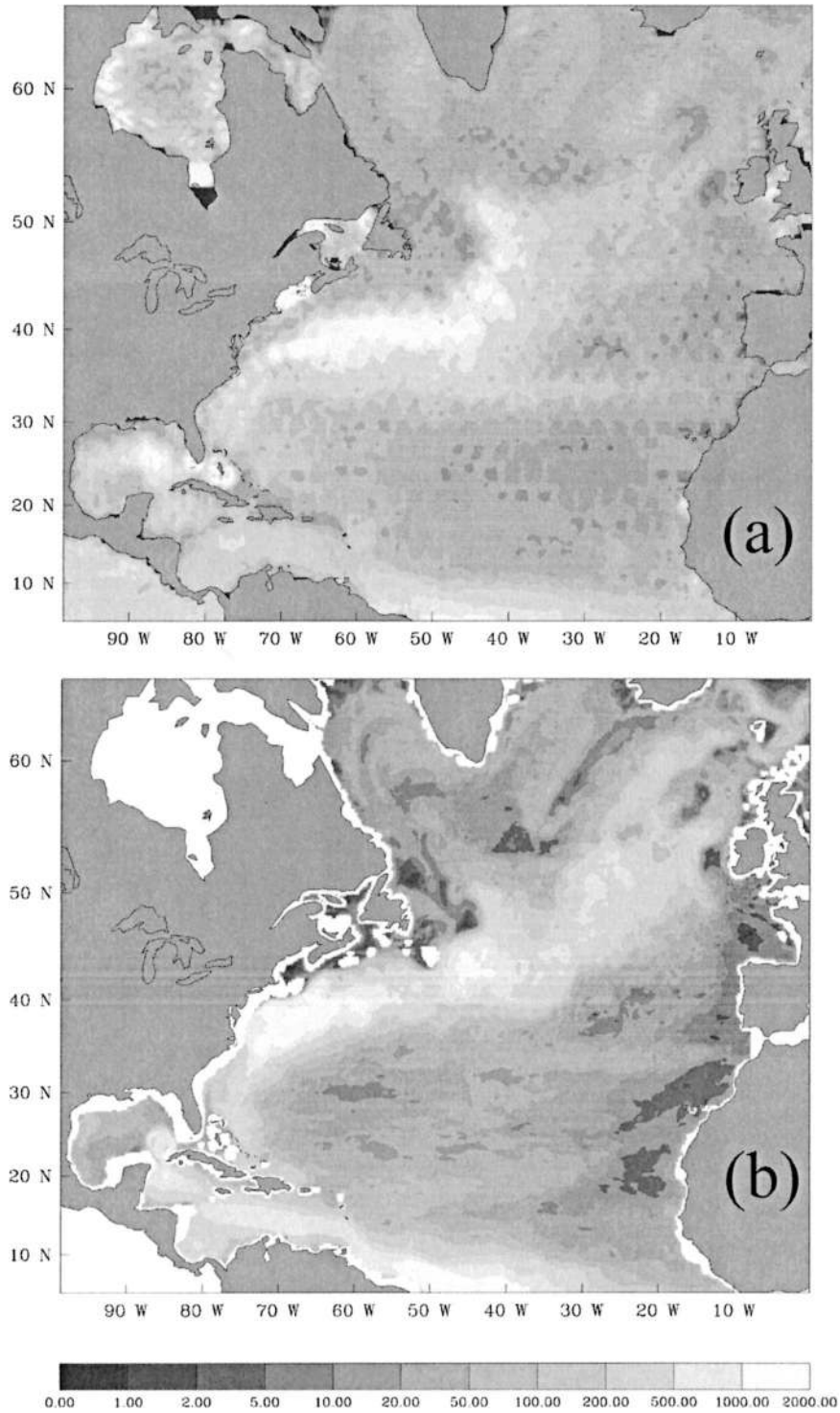
FIG. 2. Averages of yearly eddy kinetic energies (EKE; \text{cm}^2 \text{s}^{-2} ) for the period 1993–2000 from (a) TOPEX/Poseidon data and (b) the HF simulation at 55 m. Maxima in shallow regions [(a)] mostly reflect tidal errors and should not be taken into account when comparing both panels. These EKEs are computed over individual years (running EKEs on 1 Jul) and are averaged over these years. The grayscale is the same for both (a) and (b).
