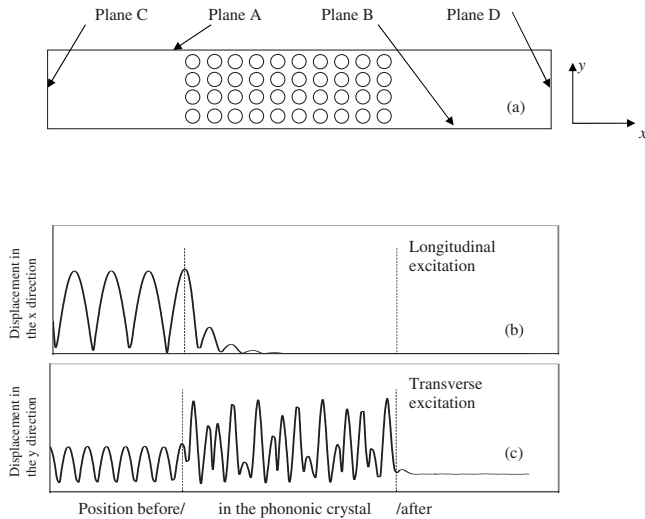
FIG. 6. (a) Schematic description of the calculated structure made of a phononic crystal slab sandwiched between two semi-infinite media. A periodic condition is applied on planes A and B. Excitation is applied on plane C. A FEM-BEM coupling is applied on planes C and D. (b) Variations in the amplitude of the displacement in the x direction as a function of the position when the excitation is a longitudinal force. (c) Variations in the amplitude of the displacement in the y direction as a function of the position when the excitation is a transverse force. The vertical dotted lines correspond to the edges of the phononic crystal slab. Amplitudes are normalized.
