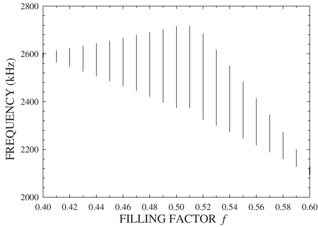
FIG. 3. Localization and width of the frequency range where negative refraction occurs vs the filling factor in the 2D phononic crystal.
