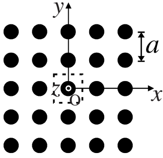
FIG. 1. Transverse cross section of the square array of cylindrical holes in a solid matrix. The holes are parallel to the z direction. The dotted lines represent the primitive unit cell of the 2D array.
