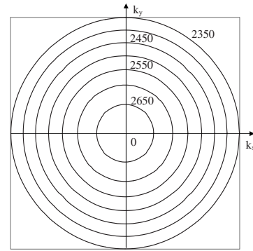
FIG. 4. EFS of the phononic crystal with 52% of air. Frequencies are varying from 2350 to 2650 kHz with 50 kHz step. The maximum values of k_x and k_y are 1.3 \text{ mm}^{-1} .
