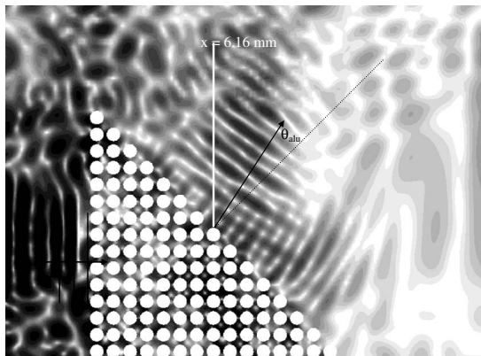
FIG. 9. Amplitude of the displacement field at t=5 \mu\text{s} . The dotted line is the normal axis to the phononic crystal. The full black line shows that a negative angle is observed when the wave is leaving the phononic crystal.
