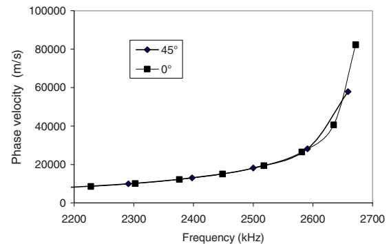
FIG. 5. (Color online) Variation in the phase velocity in the phononic crystal as a function of the frequency, for the branch with a negative slope.
