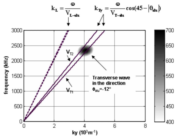
FIG. 11. (Color online) Amplitude of the displacement of the transmitted signal in the (wave number/frequency) space along the y direction. The projection along the y direction of the transverse wave numbers ( k_{Ty} = \omega \cos(45 - |\theta_{\text{alu}}|) / V_{T\text{-alu}} ) transmitted through the phononic crystal at a negative refraction angle \theta_{\text{alu}} = -12^\circ is plotted in dashed lines for the two wave velocities, in the [100] and [110] directions. Longitudinal wave numbers, in the [100] and [110] directions, are plotted in solid lines.
