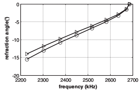
FIG. 10. Variations in the refraction angle as a function of the frequency, thanks to the Snell–Descartes law, using variations in the phase velocity from Fig. 5. The angle of incidence in the phononic crystal is equal to 45^\circ . Two transverse wave velocities are considered in aluminum: V_{T2} = 3249 \text{ m/s} (circles) and V_{T1} = 2948 \text{ m/s} (triangles).
