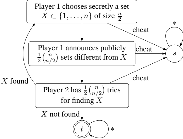
Figure 4. A game where player 2 needs a lot of memory to stay away from target state t .
