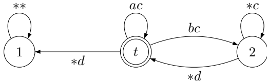
Figure 3. Co-Büchi games are not qualitatively determined.
