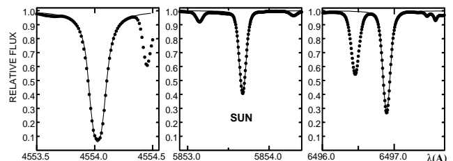
Fig. 2. Profile fitting for the barium lines in the solar spectrum with \log \epsilon(\text{Ba}) = 2.17 .
