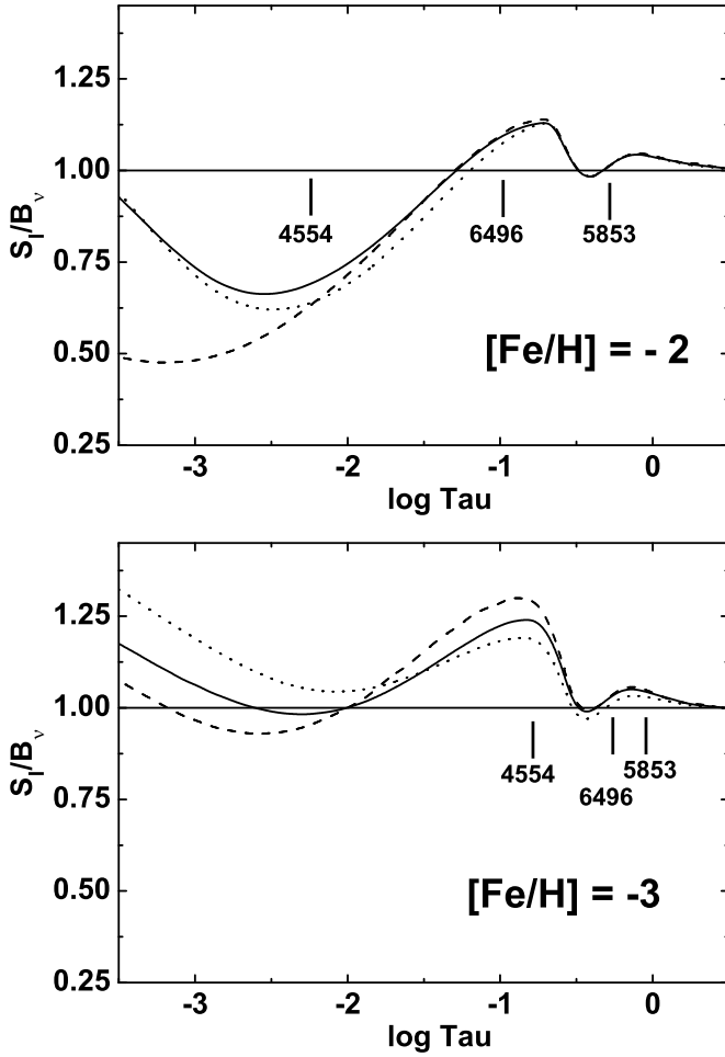
Fig. 3. Ratio S_l/B_v (Source function over Planck function) vs. the optical depth for the models T_{\text{eff}} = 5250\text{K} , \log g = 1.5 , [\text{Fe}/\text{H}] = -2.0 and -3.0 . The dashed line represents the 4554 Å line, the solid line the 5853 Å line and the dotted line the 6496 Å line.
