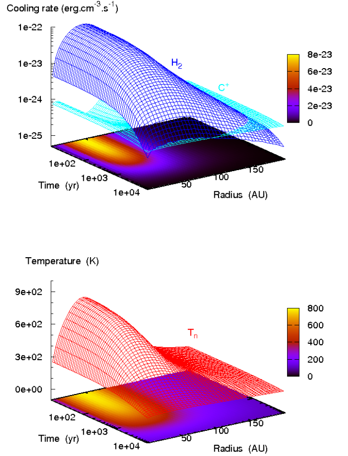
Figure 4. Vortex thermal features during the relaxation phase, as functions of the radius and time (after the vortex blow-up) for the reference model: a = 3 \times 10^{-11} \text{ s}^{-1} , n_{\text{H}} = 30 \text{ cm}^{-3} and A_{\text{V}} = 0.4 \text{ mag} . An isochoric relaxation is assumed. Top panel: the main cooling terms, i.e. the radiative desexcitation of \text{H}_2 and \text{C}^+ . Bottom panel: the temperature of the neutrals.
