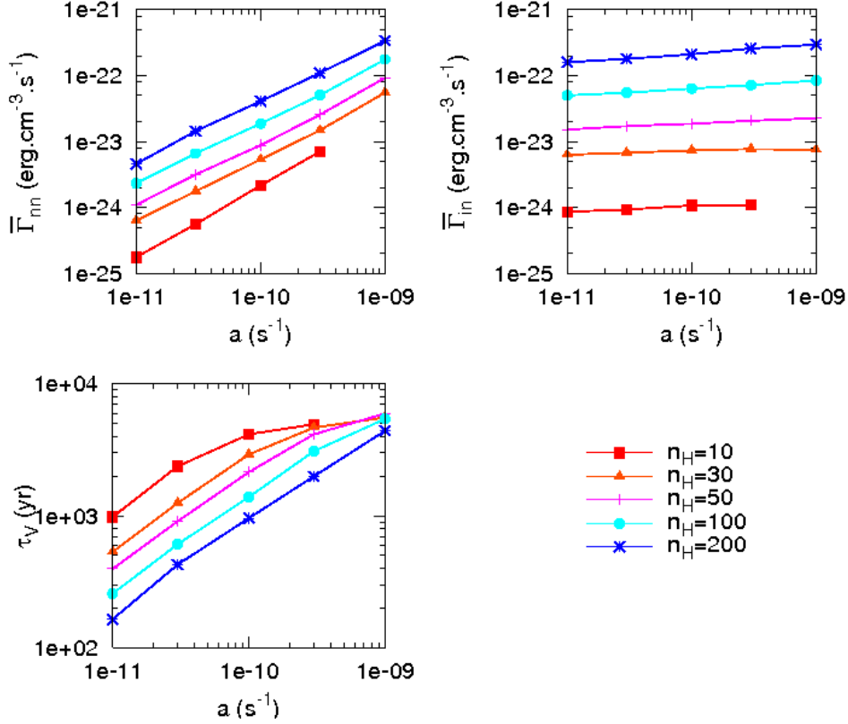
Figure 6. Main physical properties of the TDR models as functions of the turbulent rate of strain a for several values of the density n_H . Top panels: the vortex heating terms \bar{\Gamma}_{m} due to the viscous dissipation (left) and \bar{\Gamma}_{in} due to the ion-neutral friction (right). Bottom panel: the vortex lifetime \tau_V .
