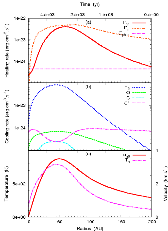
Figure 2. Vortex physical properties as functions of the radius (bottom axis) or time (top axis, arbitrary origin) for the reference model: a = 3 \times 10^{-11} \text{ s}^{-1} , n_{\text{H}} = 30 \text{ cm}^{-3} and A_V = 0.4 \text{ mag} . Panel (a): The heating terms \Gamma_{nn} due to the viscous dissipation, \Gamma_{in} due to the ion-neutral friction and \Gamma_{ph-e} due to the photoelectric effect. Panel (b): The dominant cooling terms due to the radiative desexcitation of \text{H}_2 (pure rotational lines), C, O and \text{C}^+ (fine-structure lines). Panel (c): The temperature and orthoradial velocity of the neutrals.
