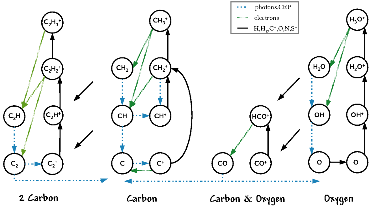
Figure C.1. Chemical network of a UV-dominated chemistry: n_H = 30 \text{ cm}^{-3} and A_V = 0.4 . This figure is simplified: for each species only the dominant reaction of production and the dominant reaction of destruction are displayed.
