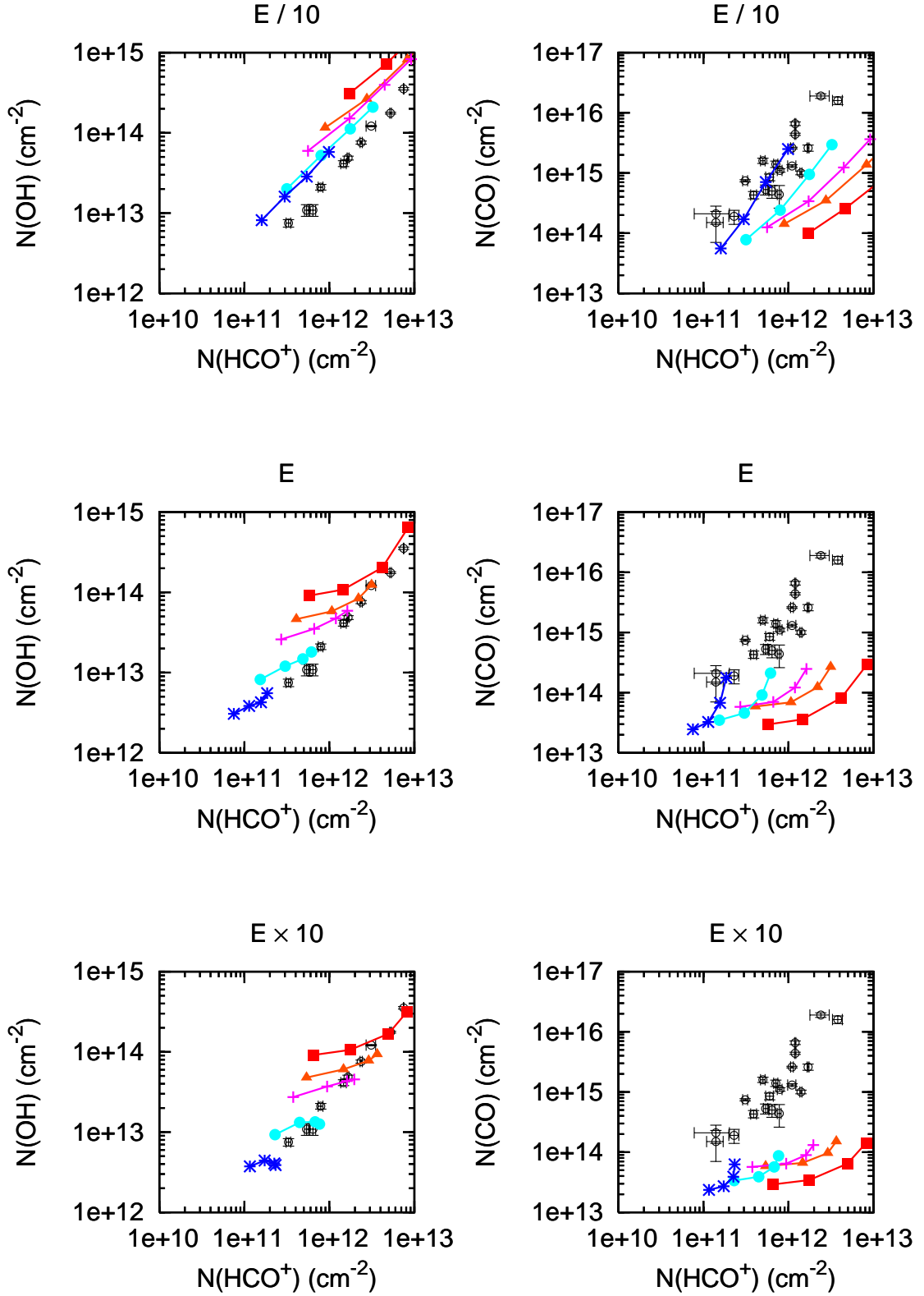
Figure B.1. Observations compared to the TDR models. The data are from Lucas & Liszt (1996) and Liszt & Lucas (1998). The TDR models are scaled to N_H = 1.8 \times 10^{21} \text{ cm}^{-2} and are computed for several values of the total energy E dissipated by a vortex: from 0.1 (top panels) to 10 times (bottom panels) that of the reference model. The symbols are the same as in Fig. 9.
