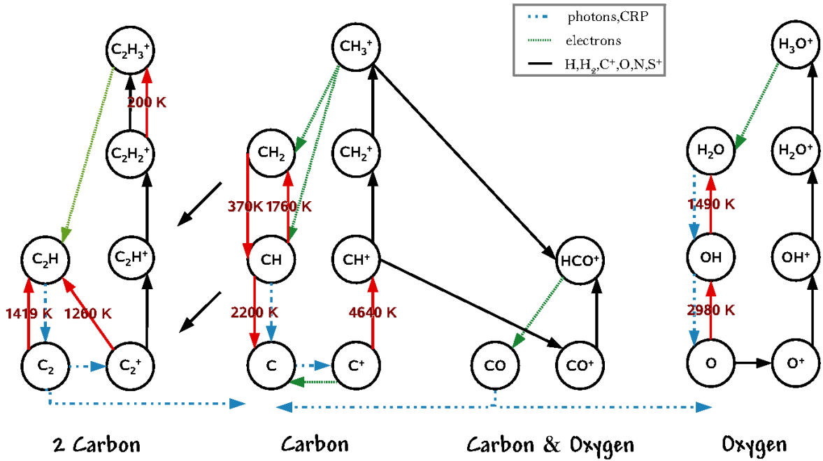
Figure C.2. Same as Fig. C.1 for a turbulence-dominated chemistry: n_H = 30 \text{ cm}^{-3} , A_V = 0.4 , a = 3 \times 10^{-11} \text{ s}^{-1} at a radius r = r_0 . The red arrows show the endoenergetic reactions with the energy involved.
