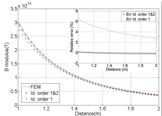
Figure 4. Magnetic field decrease (modulus) vs the distance to the source: comparison between the identified dipole/quadrupole and the actual simulated field
