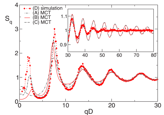
FIG. 3. (Color online) Critical S_q at the boundaries of the gel phase: Black dashed-dotted, red full, and black dashed lines mark results from (A), (B), and (C). The red diamonds indicate S_q at \phi_p=0.42 , which is close to the arrested state in the simulation (D). In the simulation, the prepeak at qD \approx 2.5 rises and shifts to smaller q values with increasing polymer concentration. The inset gives an enlarged view of the q tail where systems (A) and (B) show pronounced oscillations driven by the short-ranged attraction.
