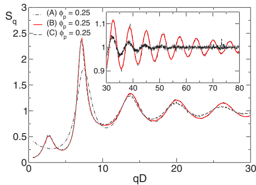
FIG. 2. (Color online) S_q from MD simulations at a colloid packing fraction of \phi_c=0.40 and a polymer concentration of \phi_p=0.25 , which is in the gel close to the critical point in MCT. The repulsive barrier affects S_q in the region below qD \leq 13 ; system (A) without barrier (dashed-dotted, black) shows neither a prepeak nor a primary peak, which is as high as in systems (B) and (C) with barrier (full red, dashed black). The inset demonstrates that polydispersity causes the q -tail oscillations in S_q to be suppressed for large wave vectors. The S_q for the polydisperse model (C) falls below the noise level for qD \geq 45 , whereas the monodisperse systems (A) and (B) virtually coincide there.
