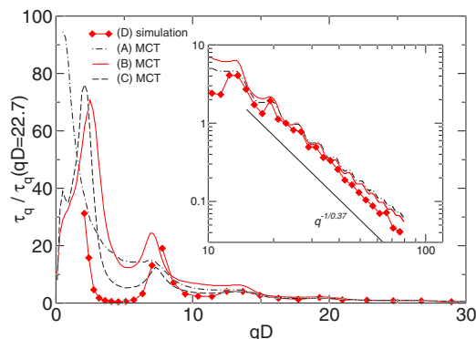
FIG. 7. (Color online) \alpha -relaxation times \tau_q in MCT for the systems (A), (B), (C) (black dashed-dotted, red full, black dashed line) and in the polydisperse simulation [(D) red diamonds]. The curves are normalized to the value of \tau_q at qD=22.7 . In the inset, the results for models (A) and (B) and simulation (D) are shown in a log-log plot. The straight line gives the asymptotic behavior \tau_q = q^{-1/b} valid for large q with the corresponding von Schweidler b = 0.37 obtained previously.
