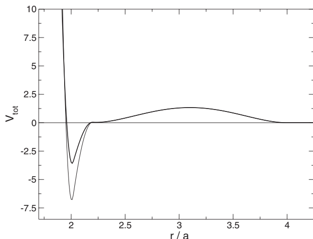
FIG. 1. Interaction potential for two particles with the average radius. The polymer fractions are \phi_p=0.42 and \phi_p=0.25 for the (lower) thin and (upper) thick curves, respectively (values close to the glass transition in the simulation and MCT, respectively). Note that in our units, the thermal energy is k_B T=4/3 .
