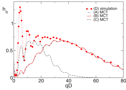
FIG. 6. (Color online) Critical amplitudes in simulation (D) (red diamonds) and MCT [(A), (B), (C)] (black dashed-dotted, red full, black dashed) close to dynamic arrest. Because of the different \alpha times in simulation and theory the MCT results for (A), (B) were scaled on the simulation results.
