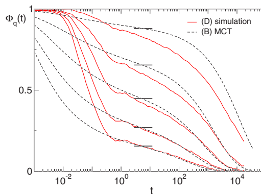
FIG. 8. (Color online) Density correlation functions in simulation [(D) red solid lines] and MCT calculations in model (B) (black dashed lines): The horizontal black bars indicate the critical plateau values of f_q^c in MCT. The wave vectors from bottom to top are qD=57.1, 45.9, 33.9, 22.7, 12.5 . The short-time diffusion coefficient was set to D^s/D^2=0.133 . The theoretical curves correspond to a polymer concentration of \phi_p=0.2461 , which means a separation parameter of about \varepsilon_{\text{MCT}}=-0.001 . The simulation results were obtained for a polymer concentration \phi_p=0.42 , which corresponds to a separation parameter of \varepsilon_{\text{simu}}=-0.015 .
