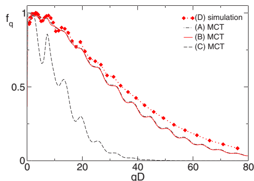
FIG. 4. (Color online) Critical nonergodicity parameters f_q^c at the transition in the simulation (D) (red diamonds), from MCT with monodisperse [(A), (B)] S_q (black dashed-dotted and red full line) and polydisperse (C) S_q (black dashed line). Serious differences occur, when the average S_q of a polydisperse system is used as input to a monodisperse theory; the shape of f_q for (C) resembles more one of a repulsive glass.
