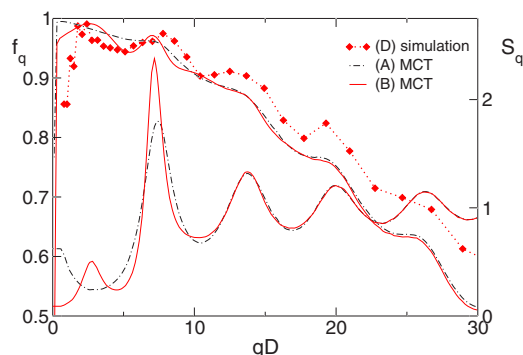
FIG. 5. (Color online) Enlarged view of the nonergodicity parameters of Fig. 4 and structure factors in the low- q region: Minor differences in f_q^c show up in the region qD \leq 10 only, where also the input S_q differs considerably. Simulation data [(D) red symbols] agree qualitatively with the model calculation (B) including the barrier.
