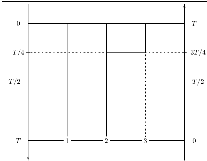
Figure 2: Interaction graph for (Z_{0:T}^1, Z_{0:T}^2)
