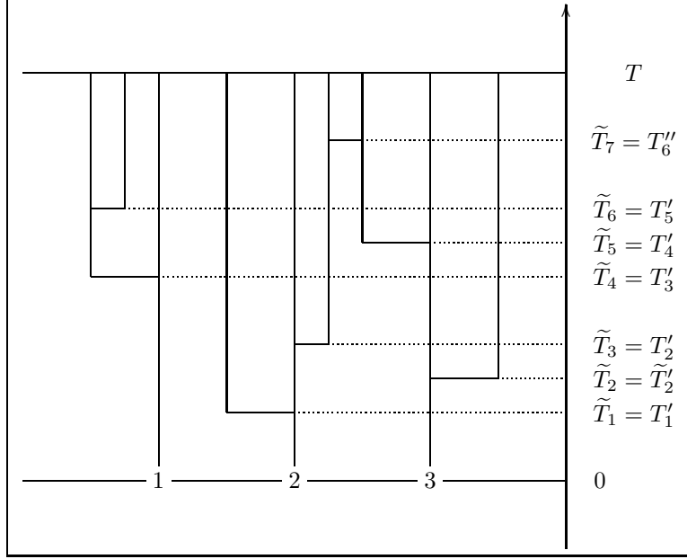
Figure 6: q = 3 , interaction graph for (\tilde{Z}_{0:T}^1, \tilde{Z}_{0:T}^2, \tilde{Z}_{0:T}^3)
