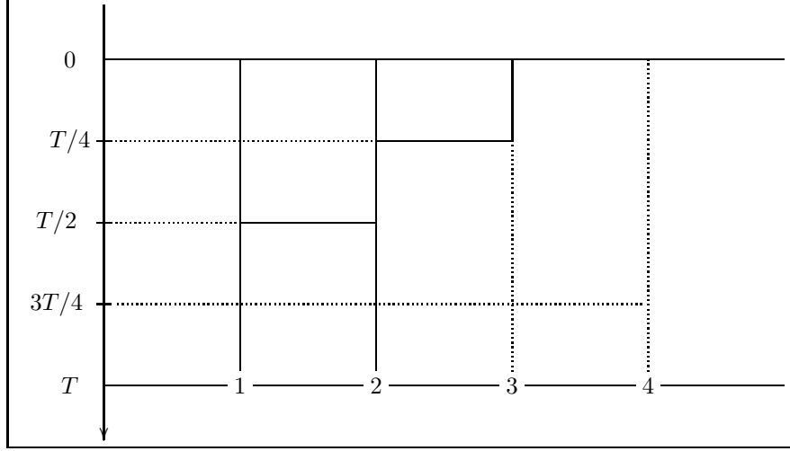
Figure 1: Interaction graph for (\overline{Z}_{0:T}^1, \overline{Z}_{0:T}^2)
