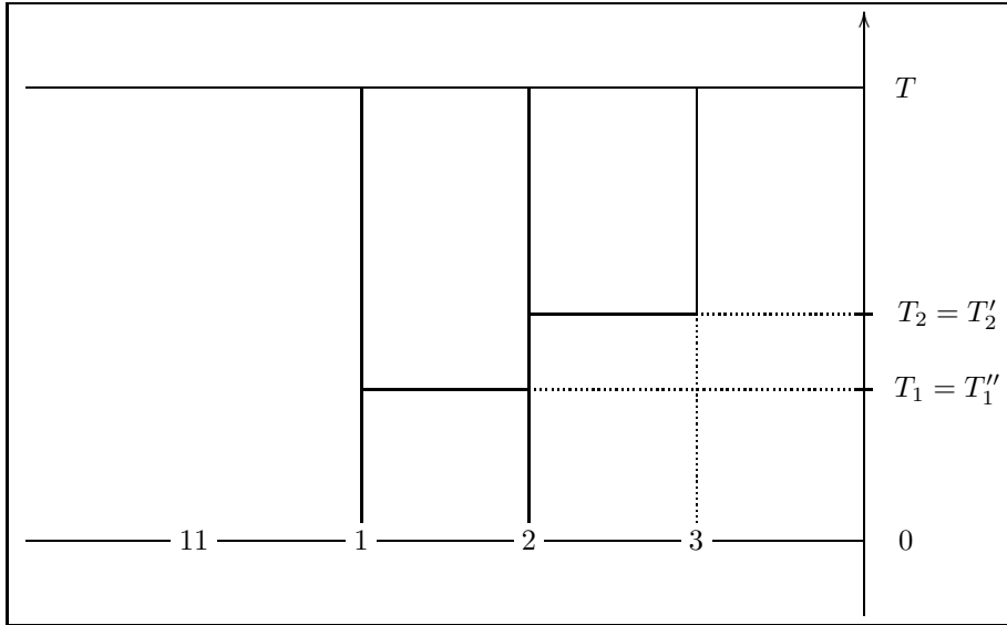
Figure 3: Interaction graph for (Z_{0:T}^{N,1}, Z_{0:T}^{N,2})
