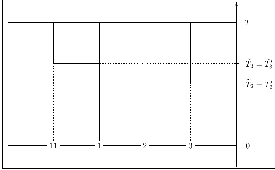
Figure 5: Interaction graph for (\tilde{Z}_{0:T}^{N,1}, \tilde{Z}_{0:T}^{N,2})
