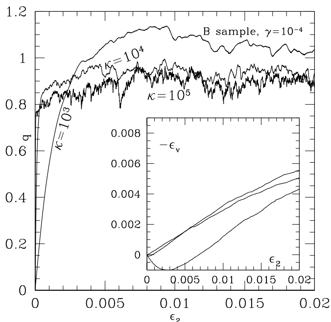
Figure 5: Results for one B-sample with 3 different stiffness values, q (main plot) and \epsilon_v (inset) vs. \epsilon_2 .
