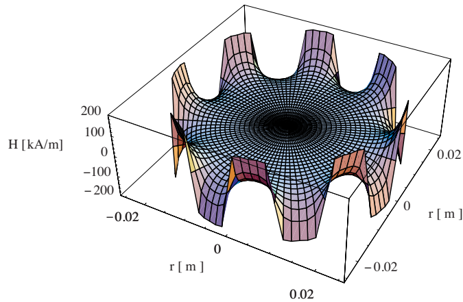
Figure 4. Three-dimensional representation of the radial field created by an alternate magnet structure: the angular width of a tile is \frac{\pi}{4} ; the inner radius is 0.025 m; the outer radius is 0.028 m; the height is 0.003 m and J = 1 T; the more H_r is calculated far from the alternate magnet structure, the thinner is the line represented in this figure ( r = 0.024 m, r = 0.023 m, r = 0.022 m), z = 0.001 m.
