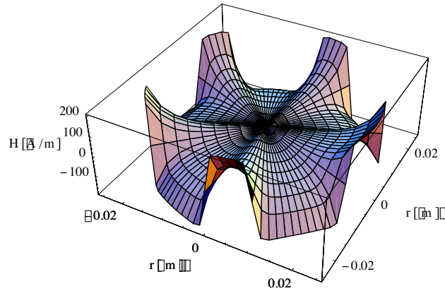
Figure 6. Three-dimensional representation of the radial field created by an alternate magnet structure whose tile permanent magnets have not the same angular width: We have \theta_2 - \theta_1 = \frac{\pi}{8} and \theta_2 - \theta_1 = \frac{\pi}{4} ; the inner radius is 0.025 m; the outer radius is 0.028 m; the height is 0.003 m and J = 1 T; the more H_r is calculated far from the alternate magnet structure, the thinner is the line represented in this figure ( r = 0.024 m, r = 0.023 m, r = 0.022 m), z = 0.001 m.
